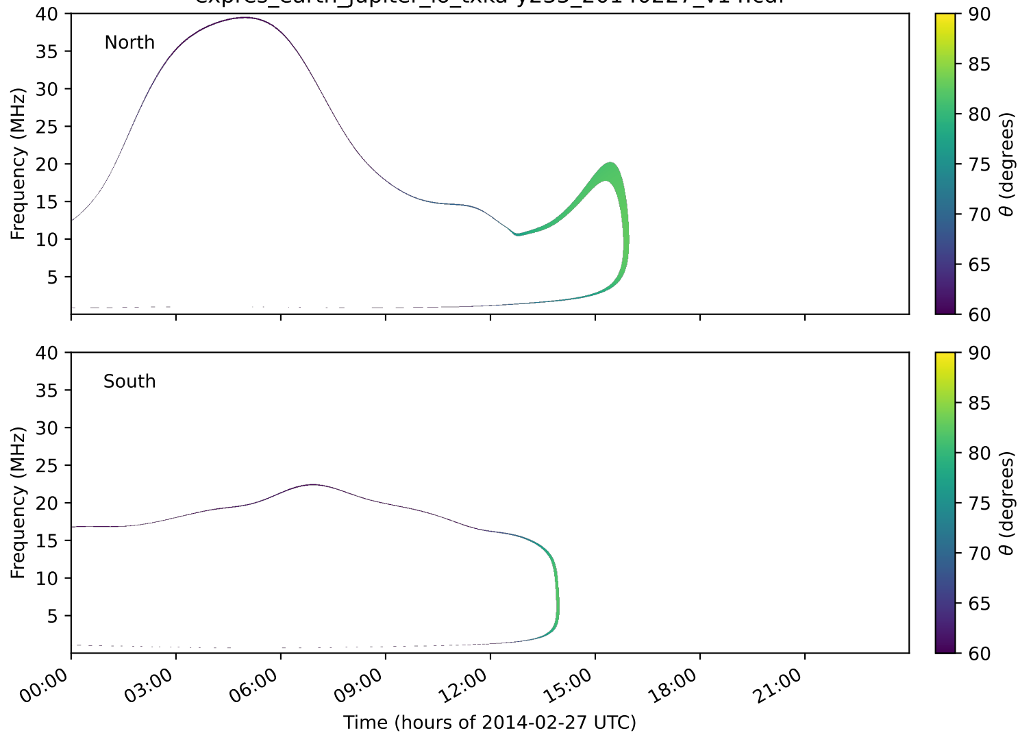
expres_earth_jupiter_io_txka-y235_20140227_v14.cdf
