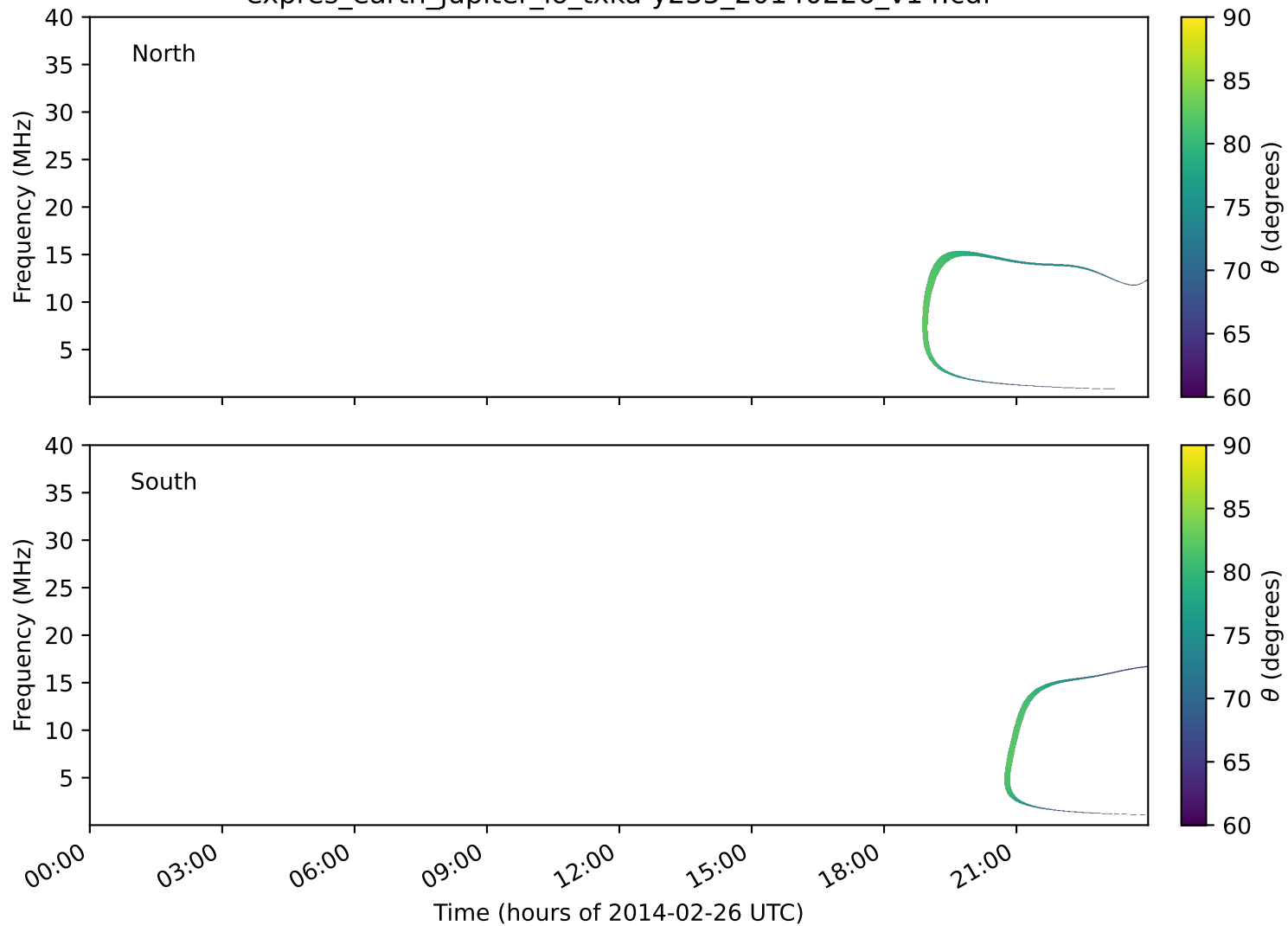
expres_earth_jupiter_io_txka-y235_20140226_v14.cdf
