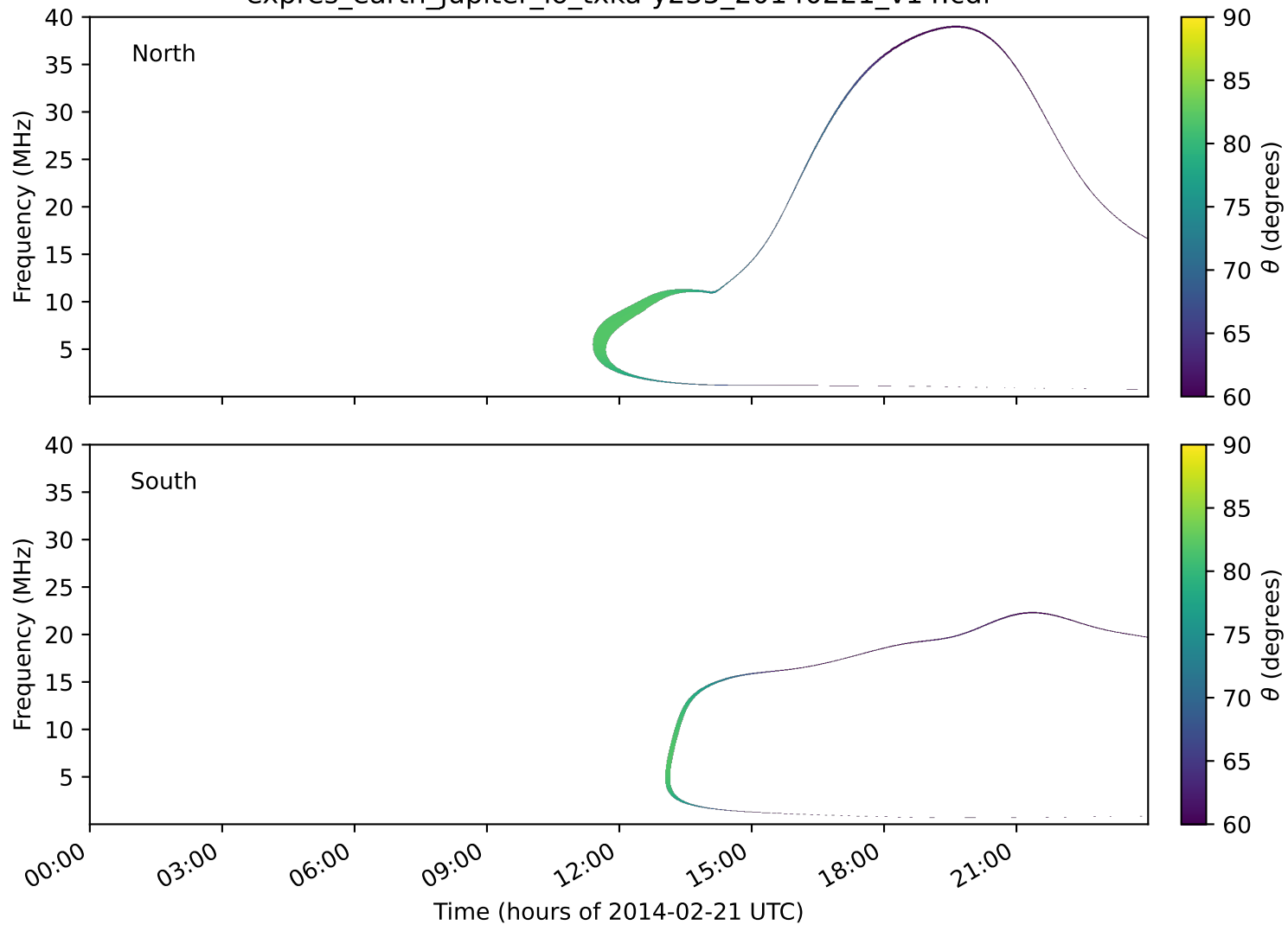
expres_earth_jupiter_io_txka-y235_20140221_v14.cdf
