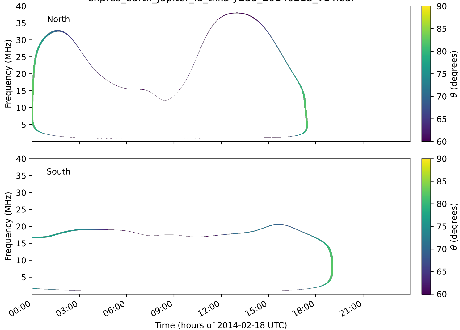
expres_earth_jupiter_io_txka-y235_20140218_v14.cdf
