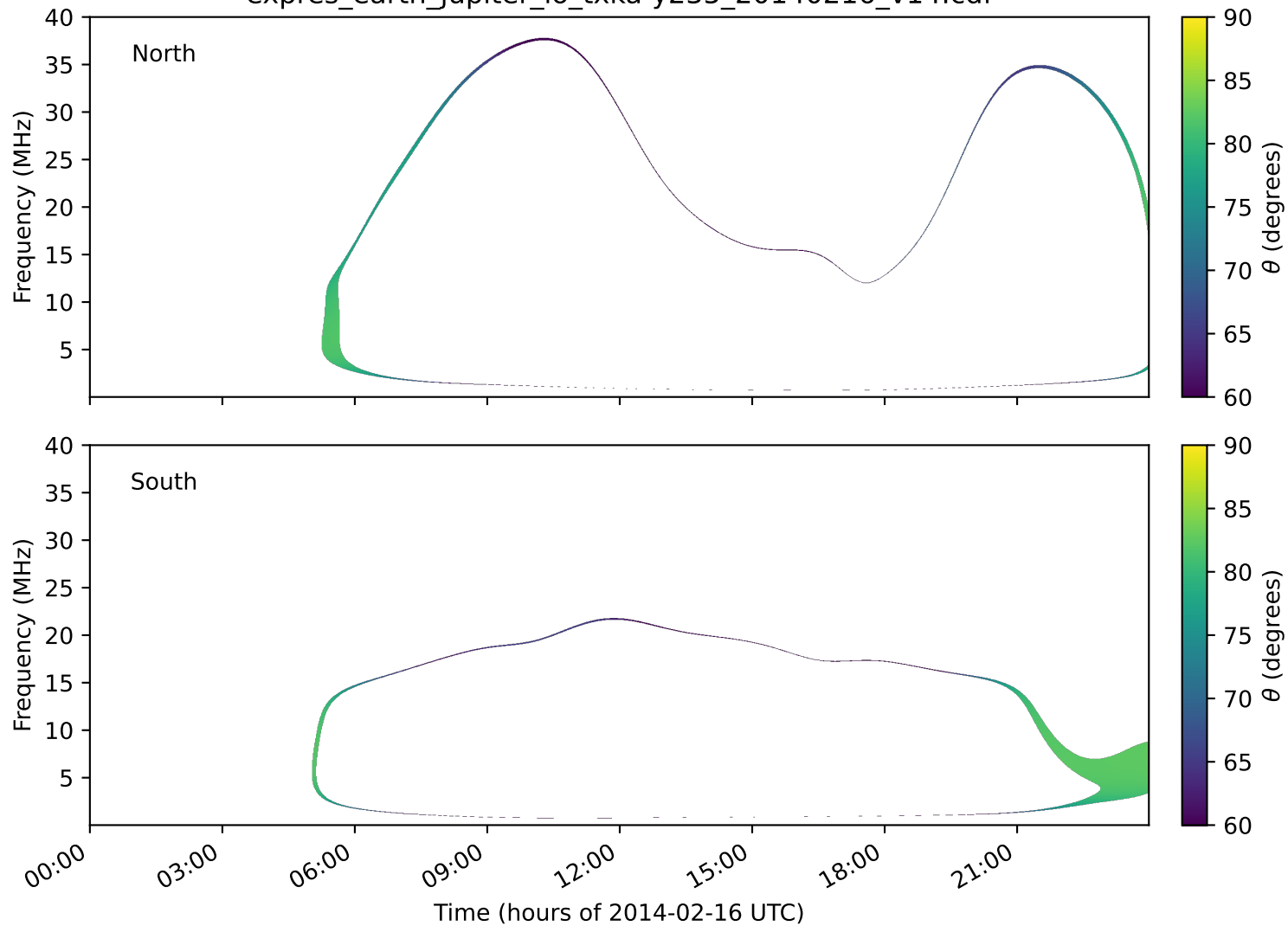
expres_earth_jupiter_io_txka-y235_20140216_v14.cdf
