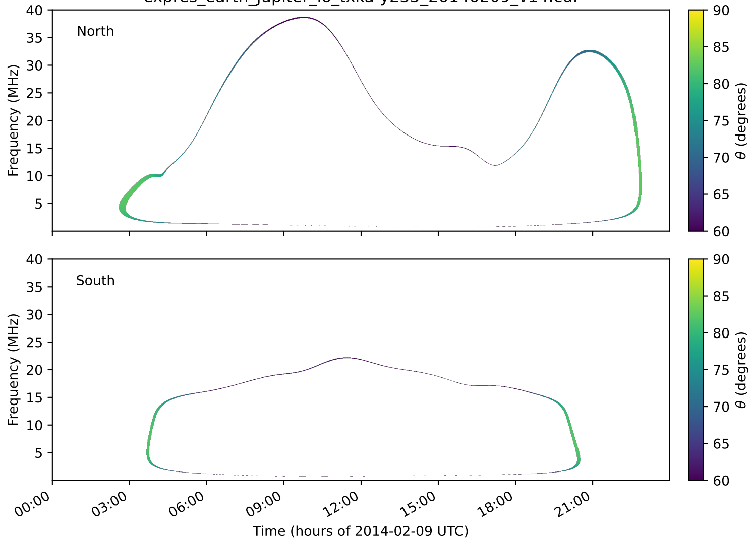
expres_earth_jupiter_io_txka-y235_20140209_v14.cdf
