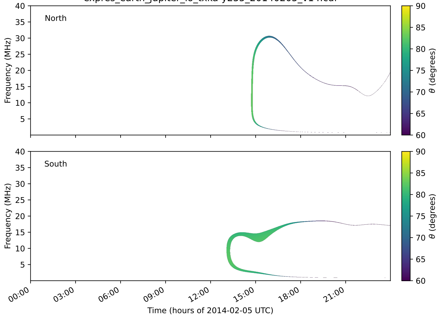
expres_earth_jupiter_io_txka-y235_20140205_v14.cdf
