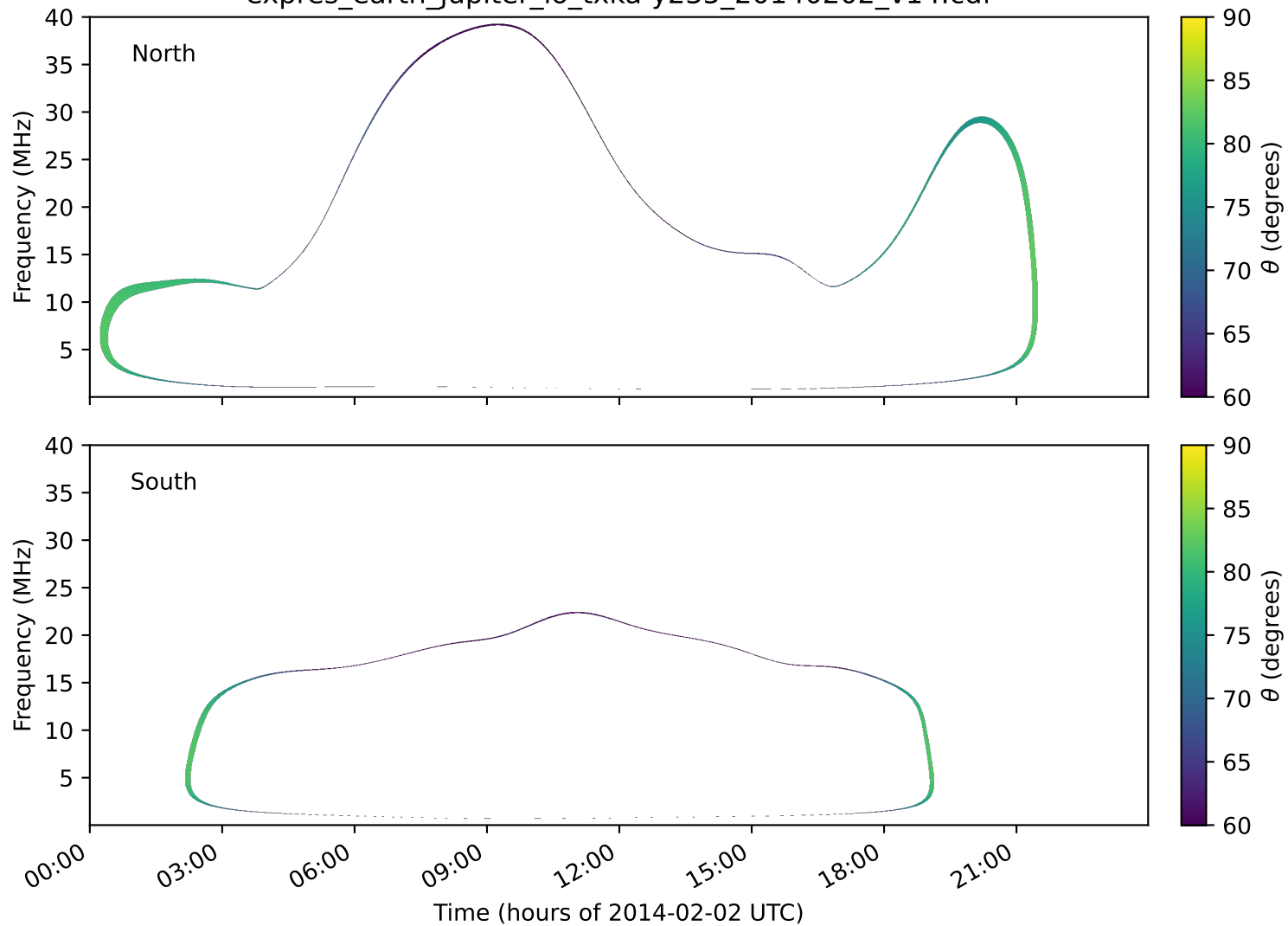
expres_earth_jupiter_io_txka-y235_20140202_v14.cdf
