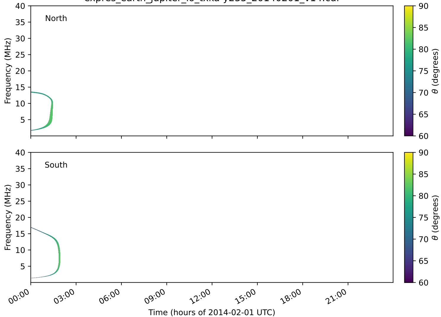
expres_earth_jupiter_io_txka-y235_20140201_v14.cdf
