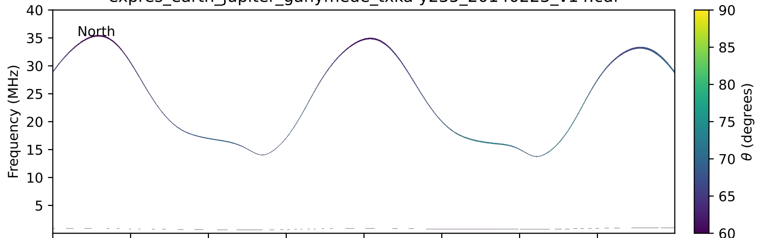
expres_earth_jupiter_ganymede_txka-y235_20140223_v14.cdf
