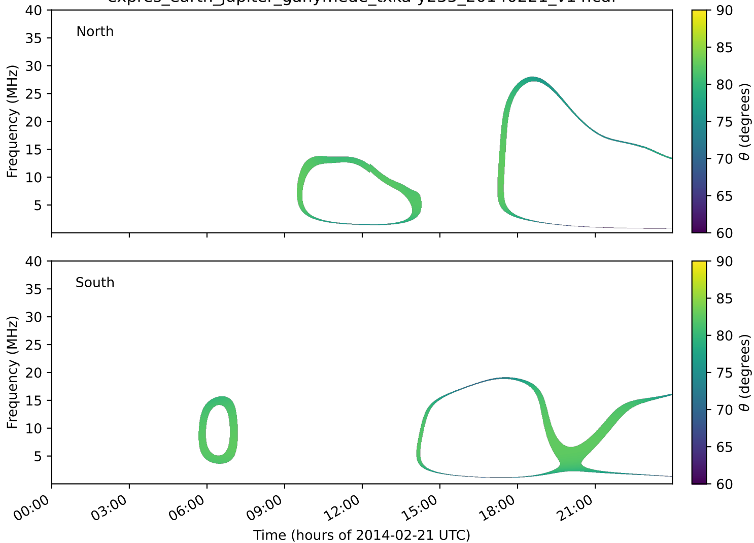
expres_earth_jupiter_ganymede_txka-y235_20140221_v14.cdf
