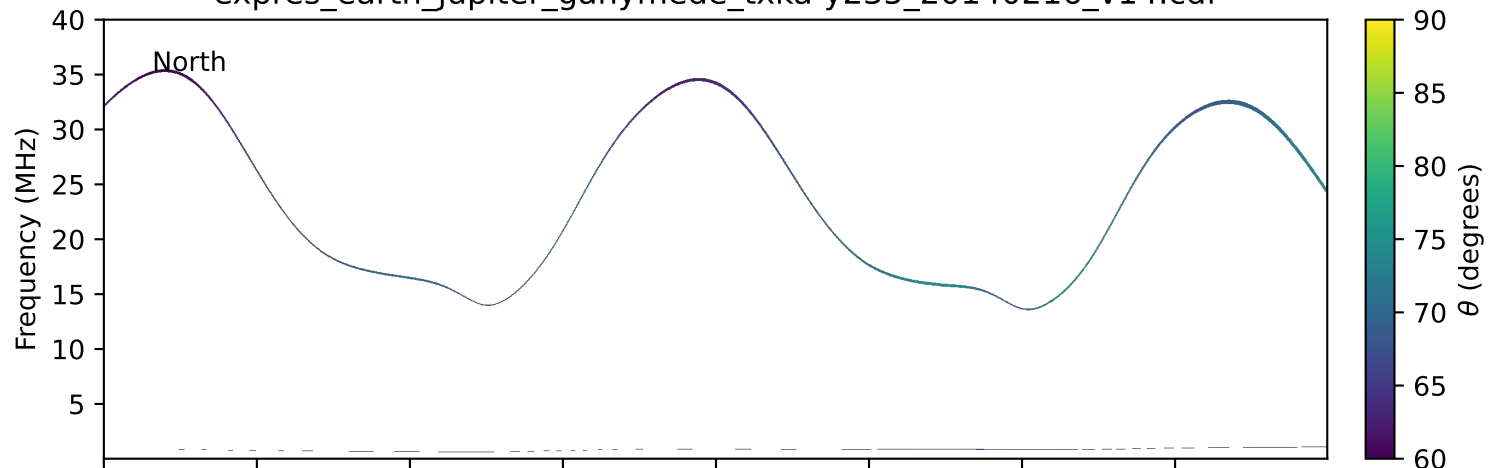
expres_earth_jupiter_ganymede_txka-y235_20140216_v14.cdf
