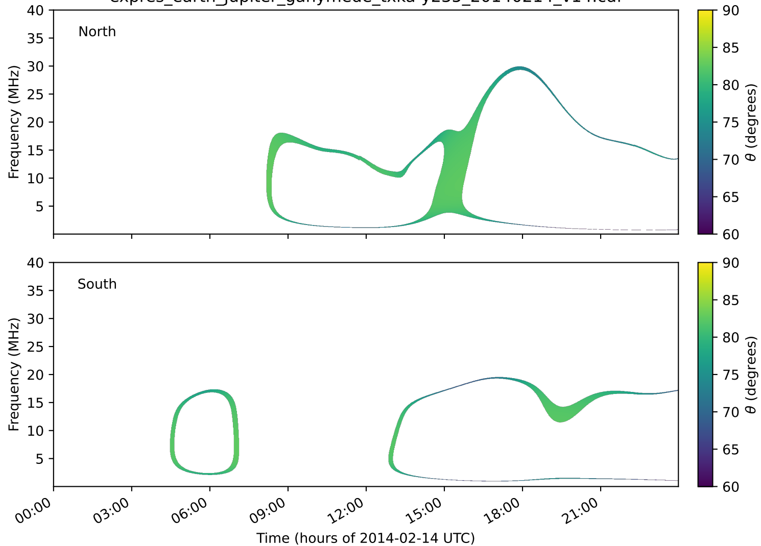
expres_earth_jupiter_ganymede_txka-y235_20140214_v14.cdf
