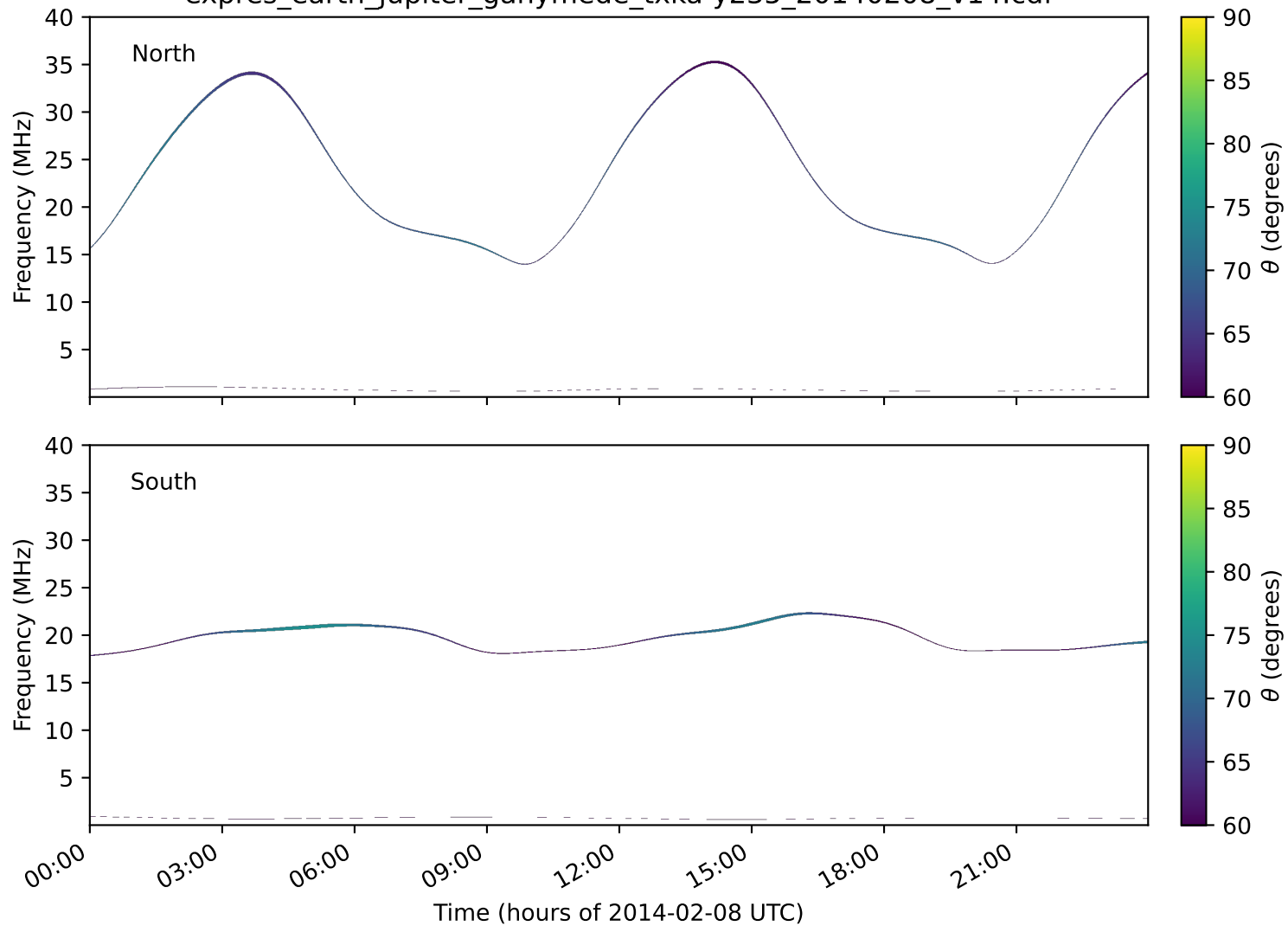
expres_earth_jupiter_ganymede_txka-y235_20140208_v14.cdf
