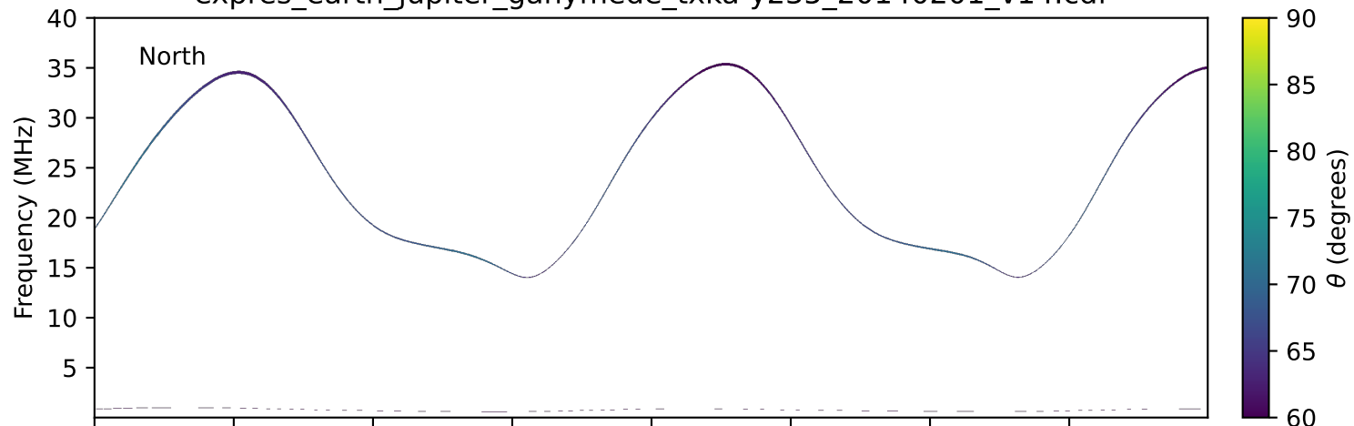
expres_earth_jupiter_ganymede_txka-y235_20140201_v14.cdf
