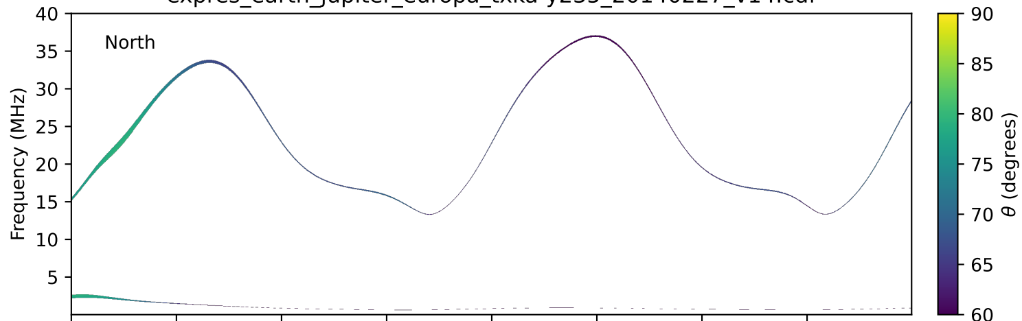
expres_earth_jupiter_europa_txka-y235_20140227_v14.cdf
