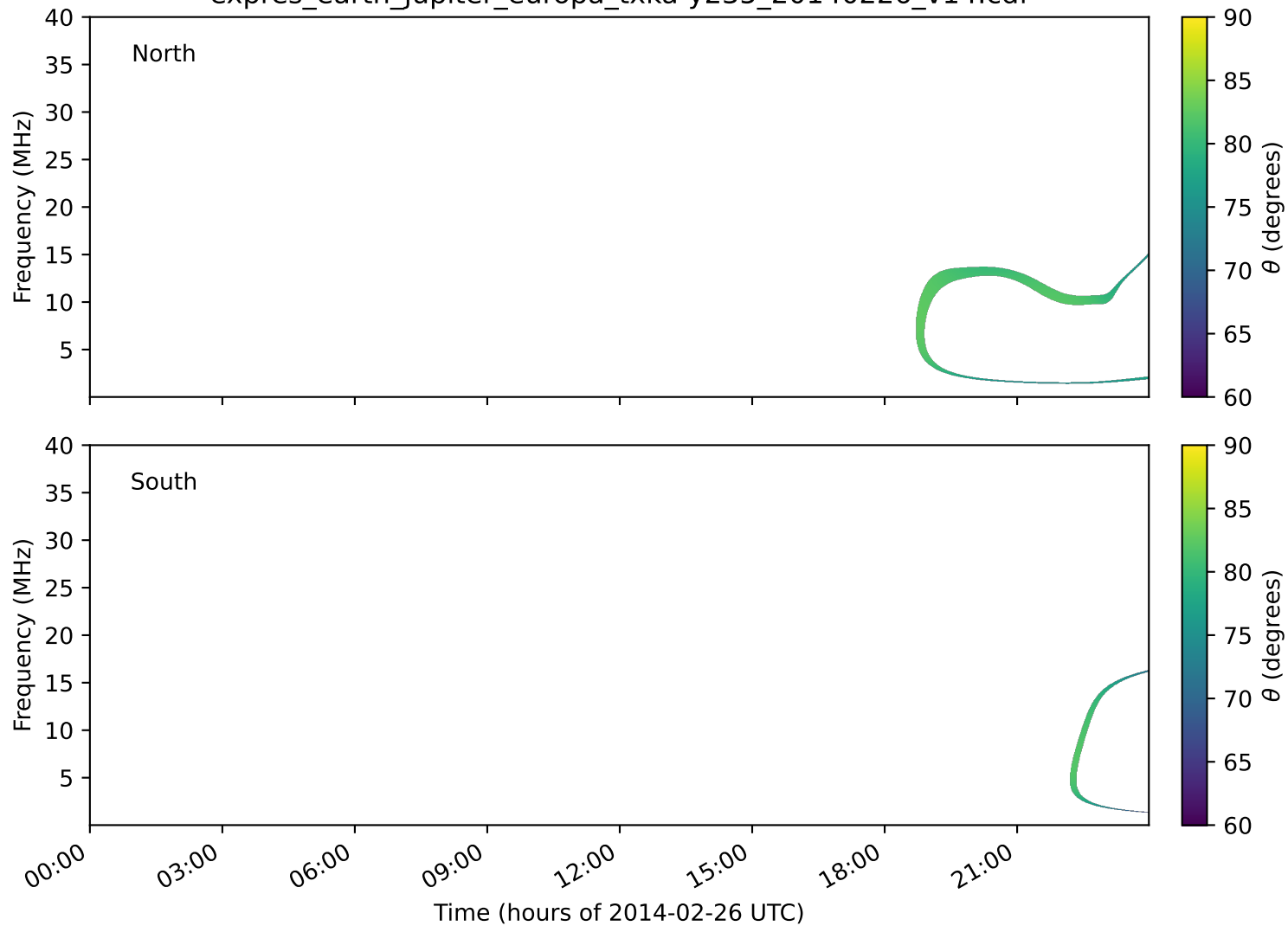
expres_earth_jupiter_europa_txka-y235_20140226_v14.cdf
