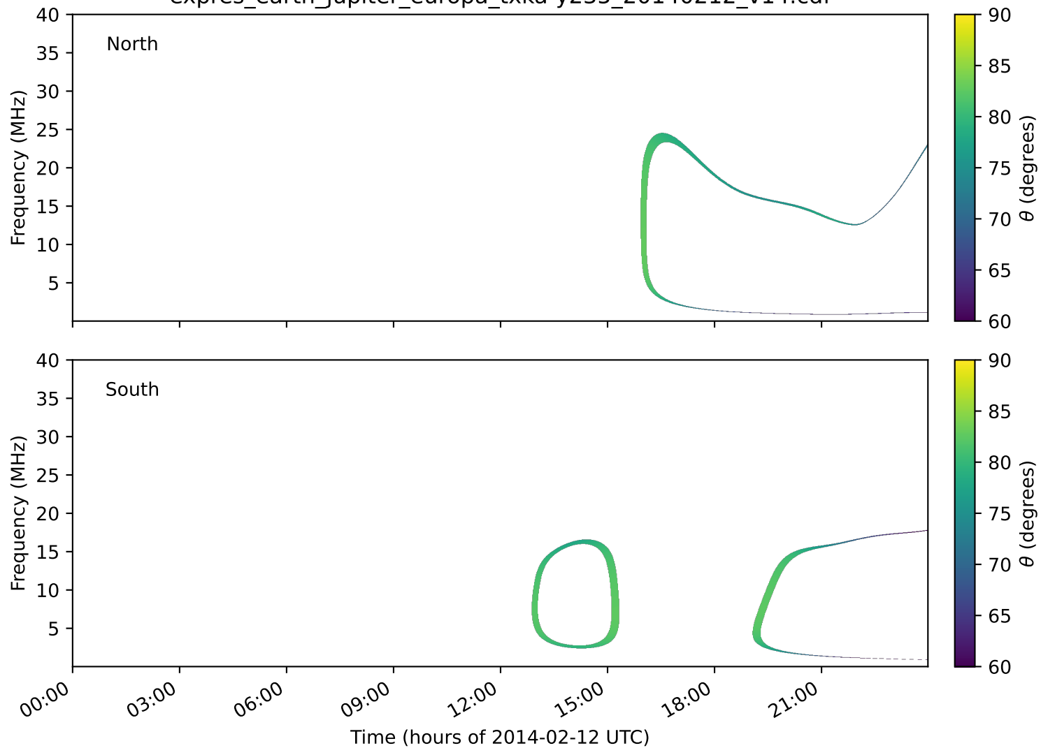
expres_earth_jupiter_europa_txka-y235_20140212_v14.cdf
