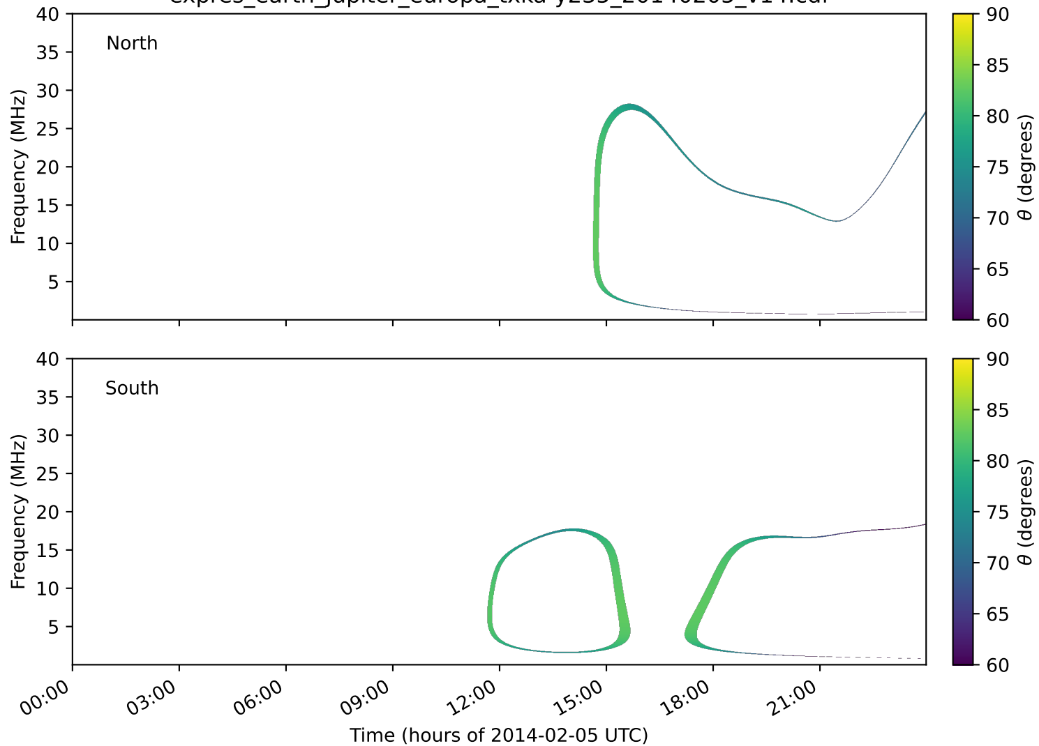
expres_earth_jupiter_europa_txka-y235_20140205_v14.cdf
