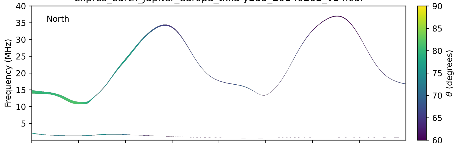
expres_earth_jupiter_europa_txka-y235_20140202_v14.cdf
