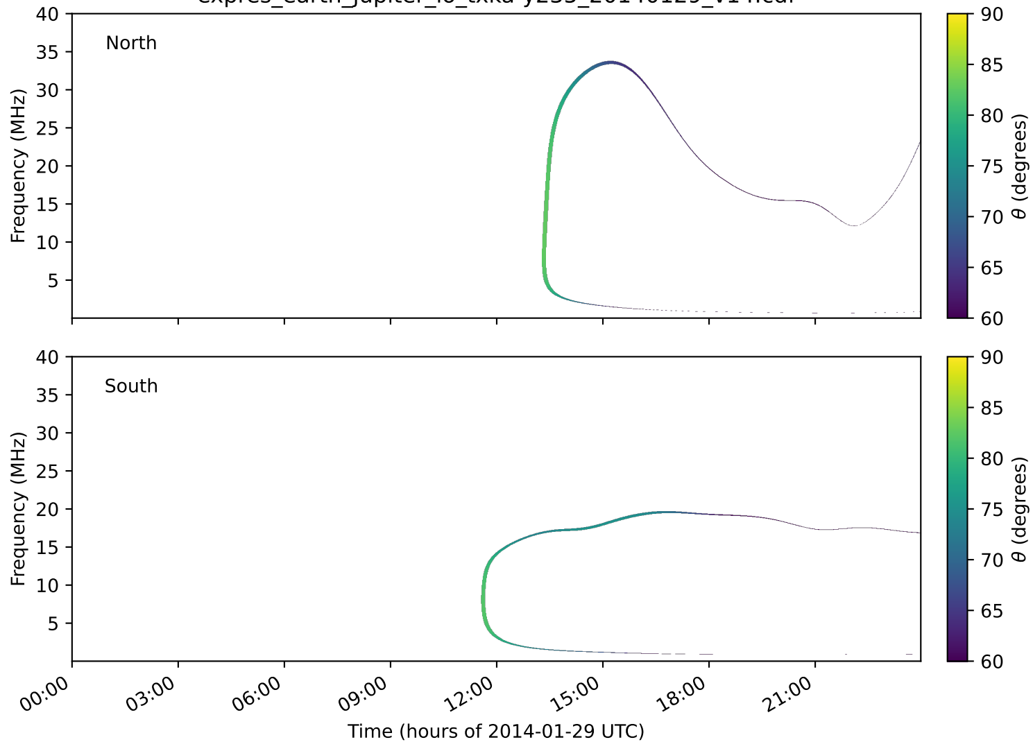
expres_earth_jupiter_io_txka-y235_20140129_v14.cdf
