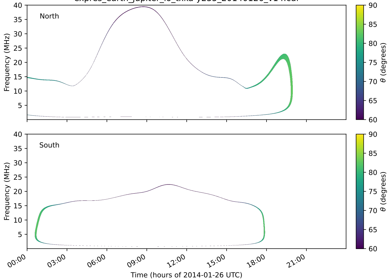
expres_earth_jupiter_io_txka-y235_20140126_v14.cdf
