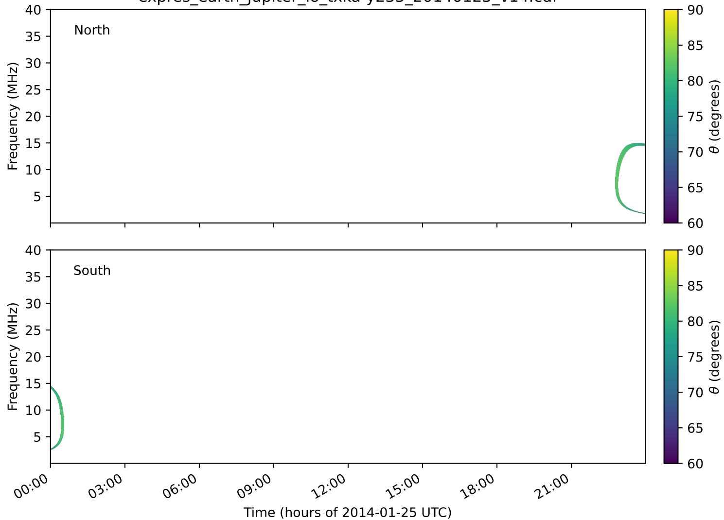
expres_earth_jupiter_io_txka-y235_20140125_v14.cdf
