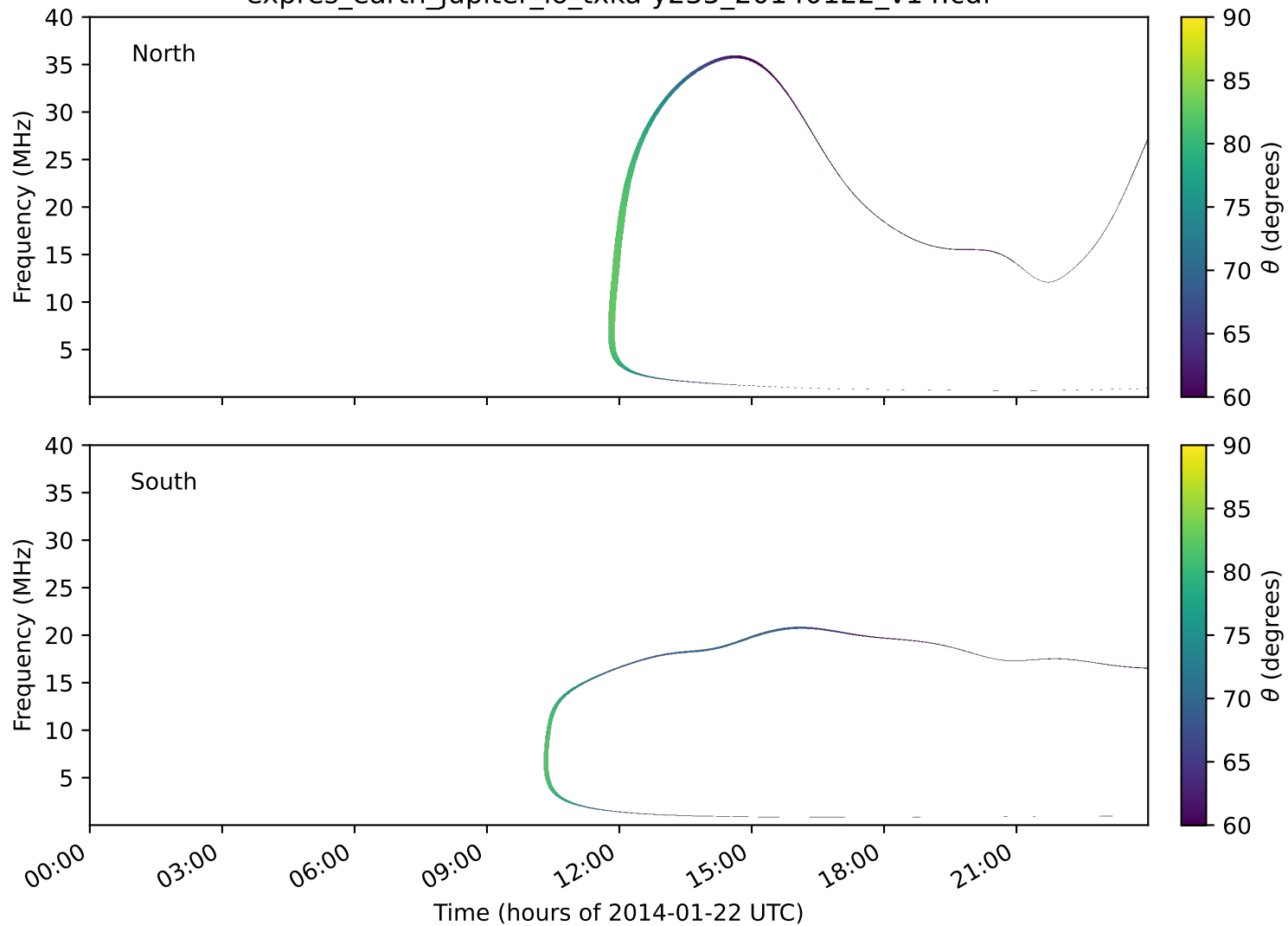
expres_earth_jupiter_io_txka-y235_20140122_v14.cdf
