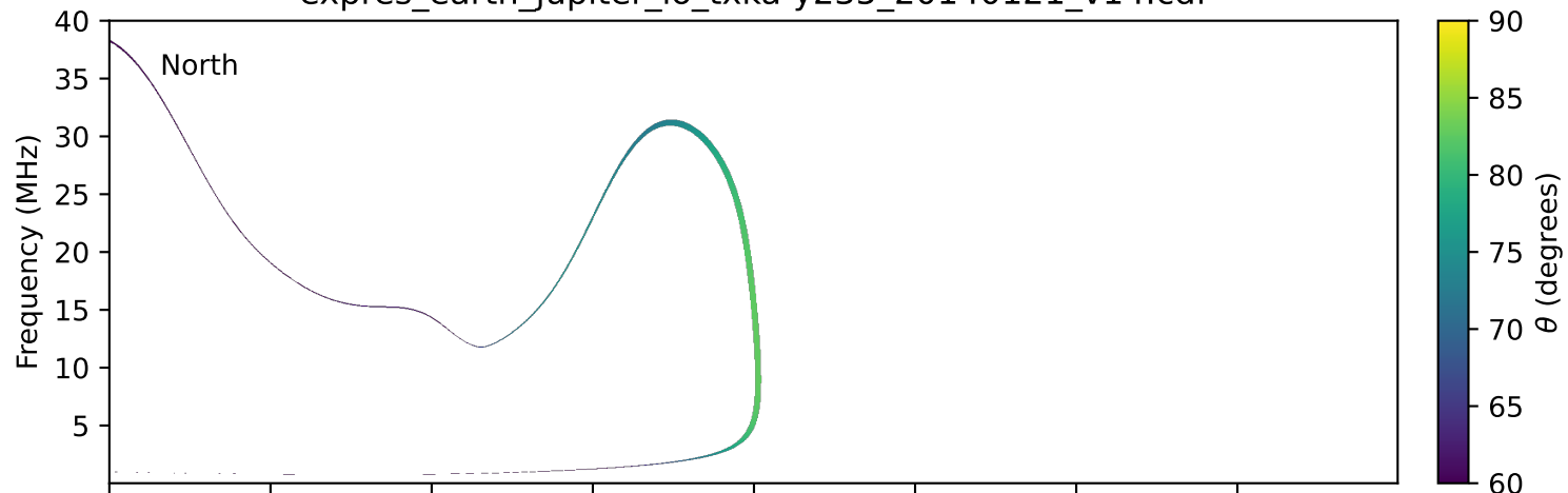
expres_earth_jupiter_io_txka-y235_20140121_v14.cdf
