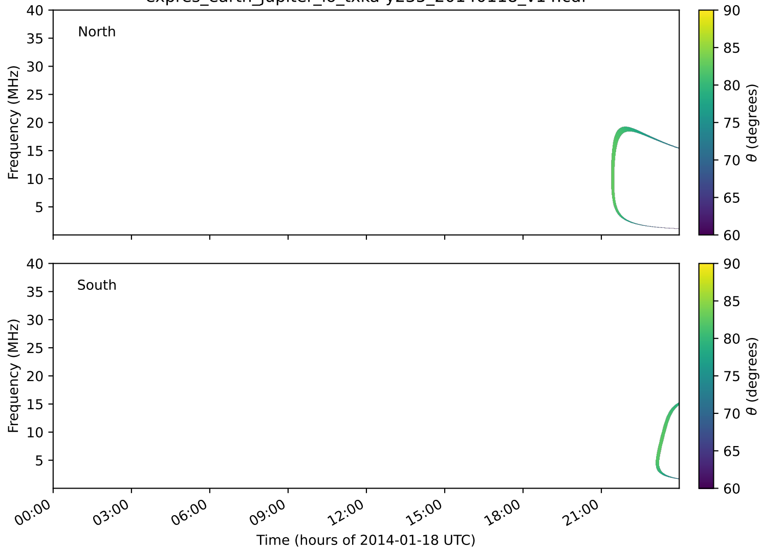
expres_earth_jupiter_io_txka-y235_20140118_v14.cdf
