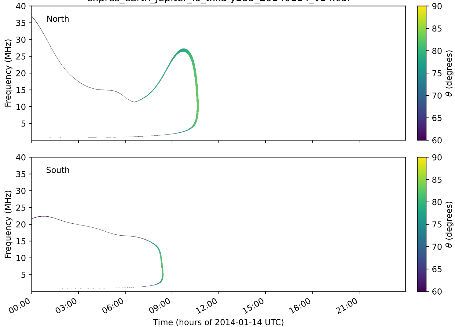
expres_earth_jupiter_io_txka-y235_20140114_v14.cdf
