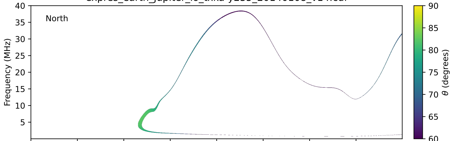
expres_earth_jupiter_io_txka-y235_20140108_v14.cdf
