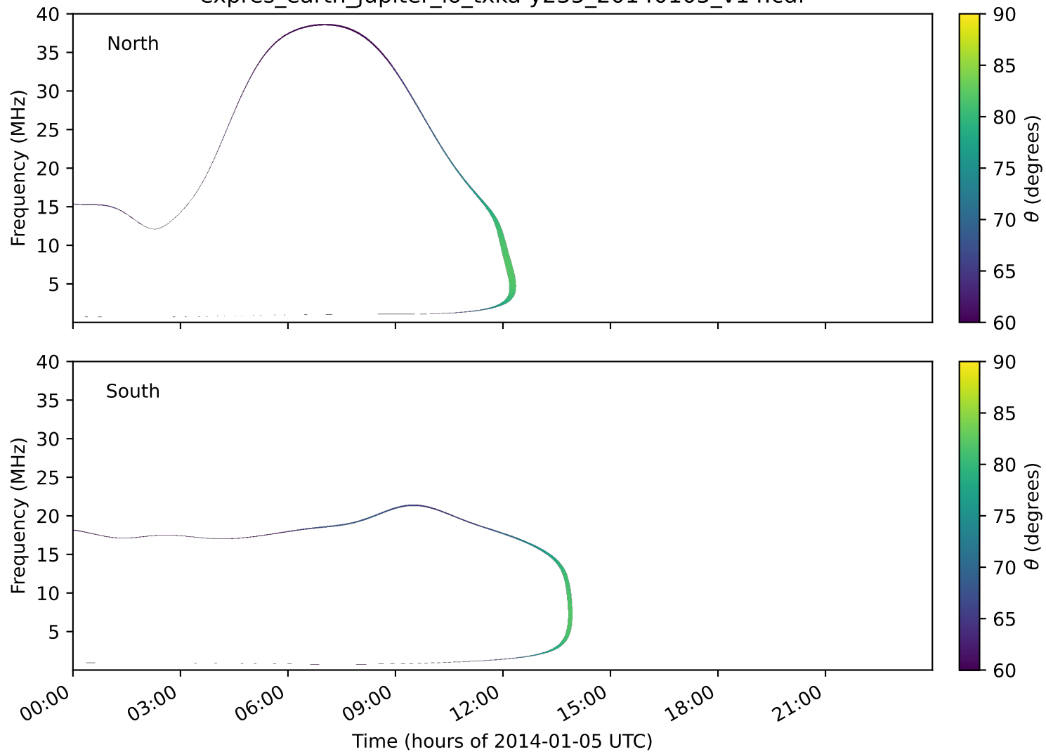
expres_earth_jupiter_io_txka-y235_20140105_v14.cdf
