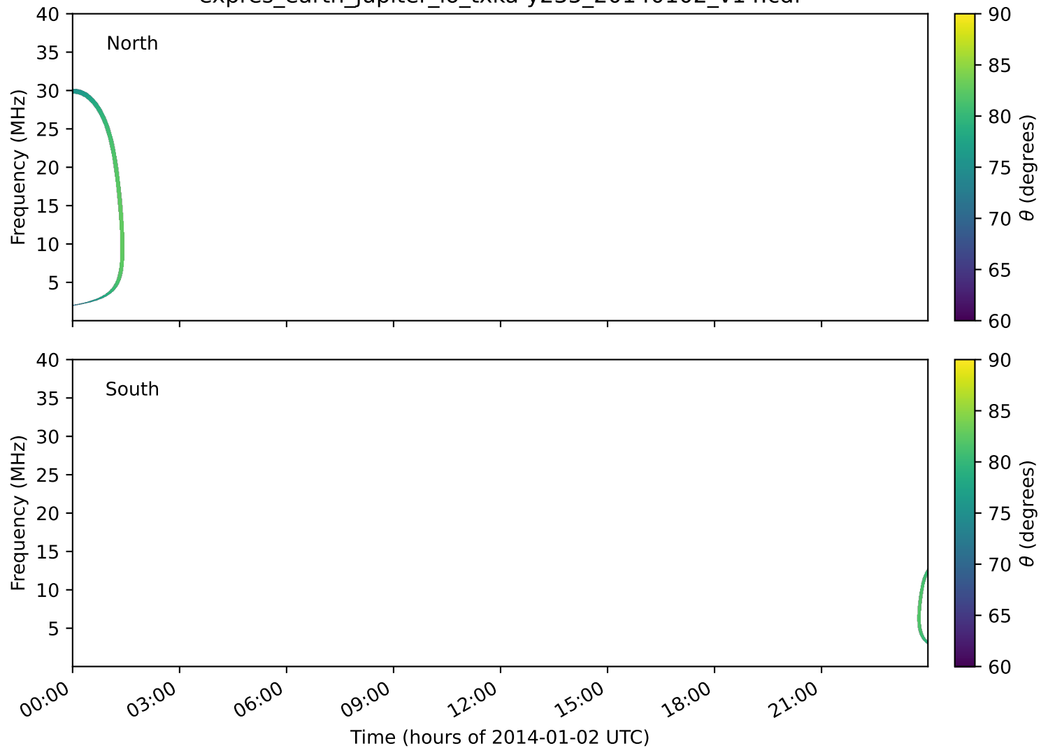
expres_earth_jupiter_io_txka-y235_20140102_v14.cdf
