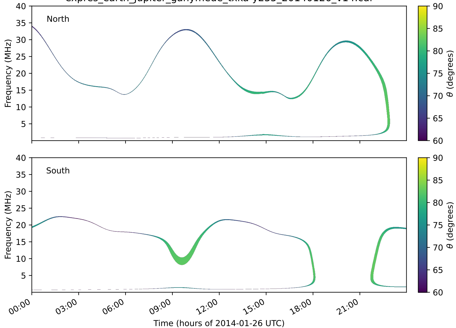
expres_earth_jupiter_ganymede_txka-y235_20140126_v14.cdf
