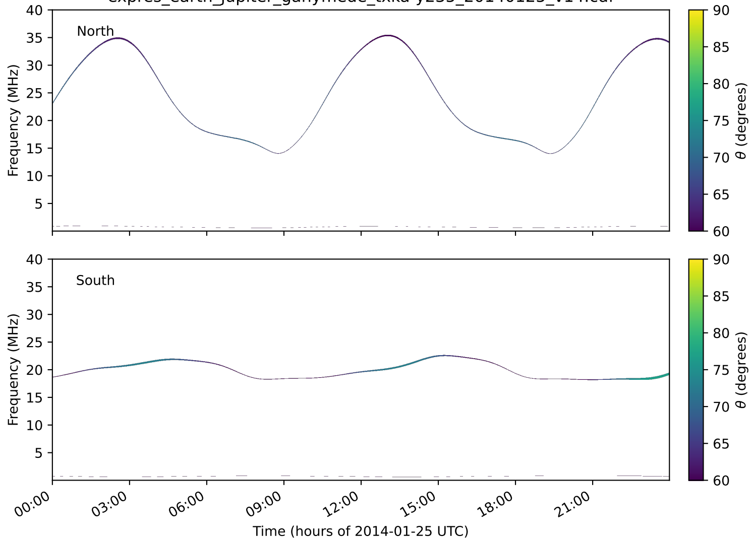
expres_earth_jupiter_ganymede_txka-y235_20140125_v14.cdf
