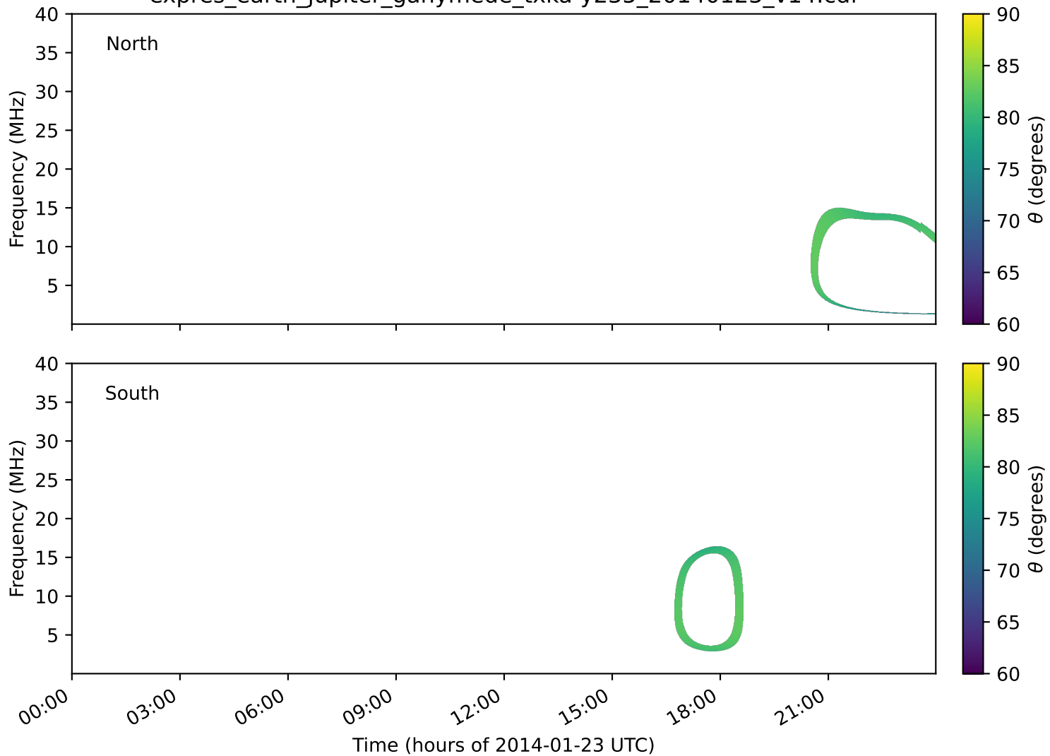
expres_earth_jupiter_ganymede_txka-y235_20140123_v14.cdf
