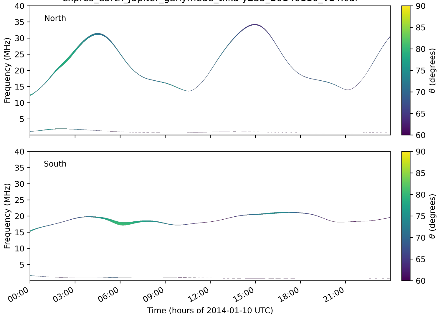
expres_earth_jupiter_ganymede_txka-y235_20140110_v14.cdf
