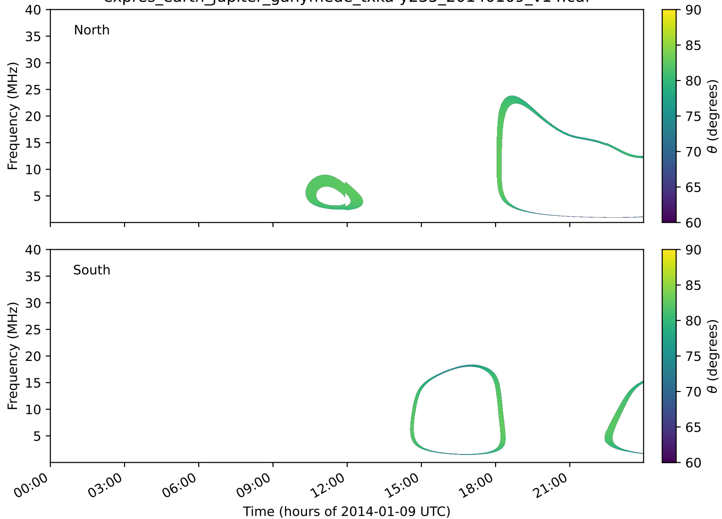
expres_earth_jupiter_ganymede_txka-y235_20140109_v14.cdf
