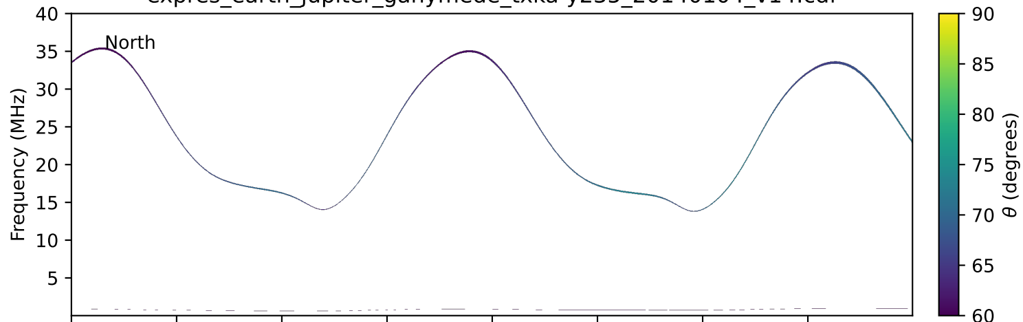
expres_earth_jupiter_ganymede_txka-y235_20140104_v14.cdf
