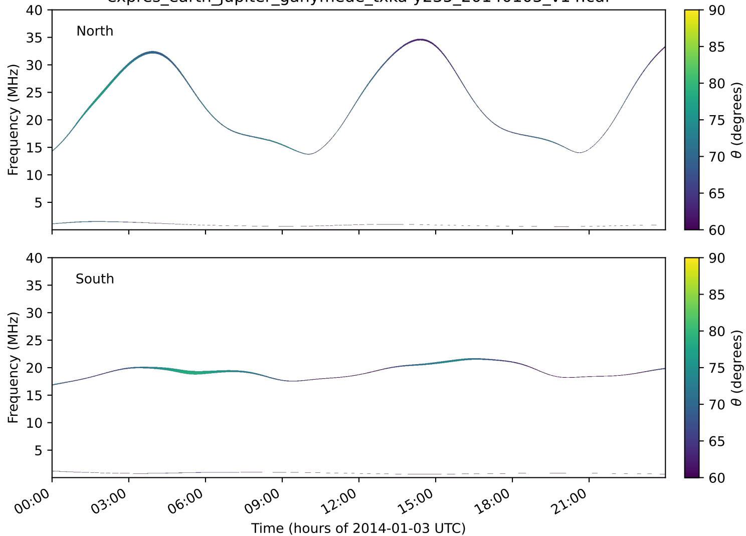
expres_earth_jupiter_ganymede_txka-y235_20140103_v14.cdf
