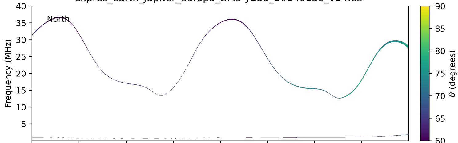
expres_earth_jupiter_europa_txka-y235_20140130_v14.cdf
