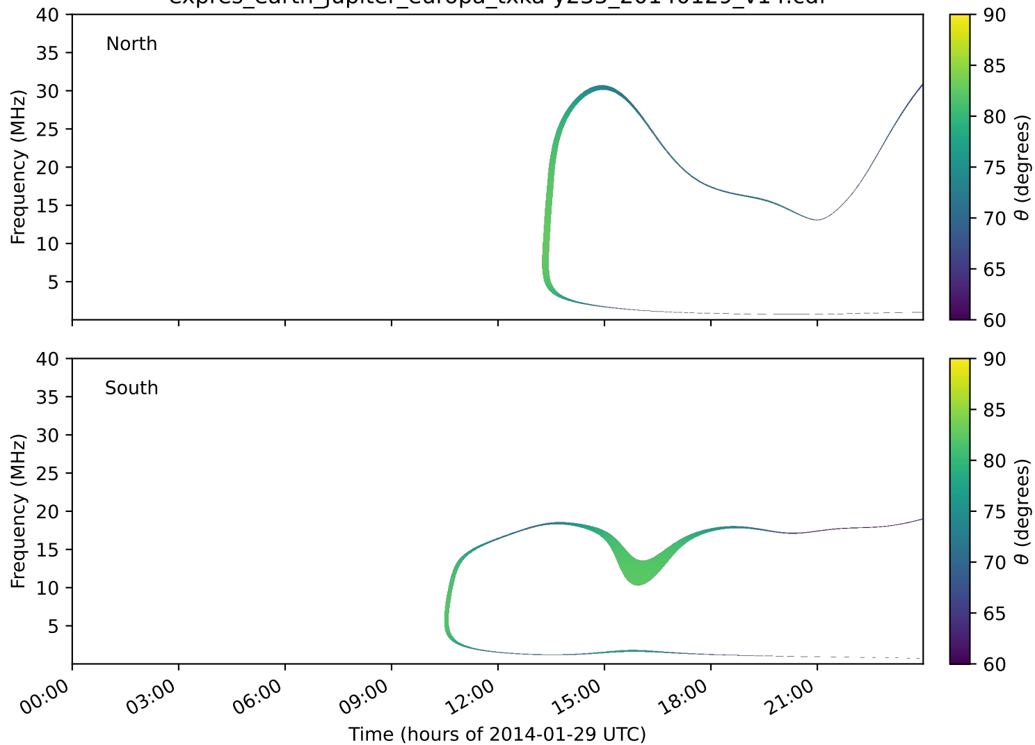
expres_earth_jupiter_europa_txka-y235_20140129_v14.cdf
