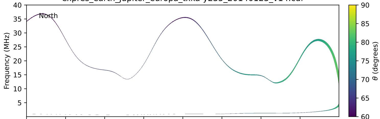
expres_earth_jupiter_europa_txka-y235_20140123_v14.cdf
