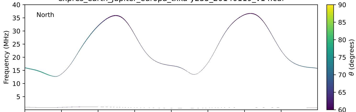
expres_earth_jupiter_europa_txka-y235_20140119_v14.cdf
