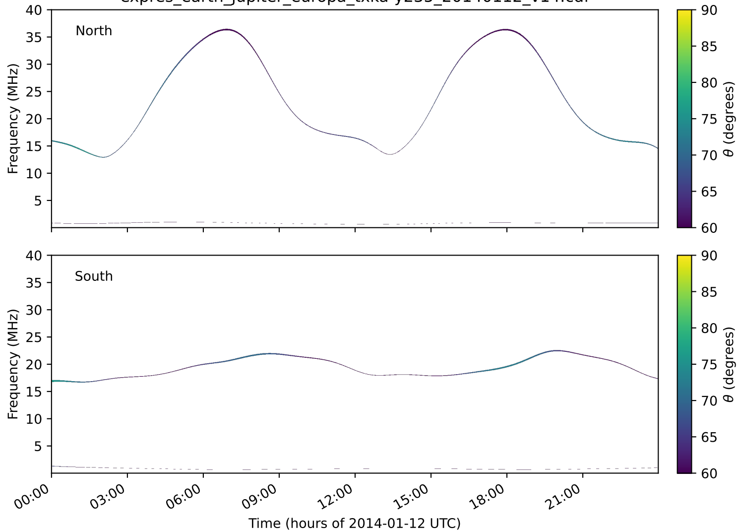
expres_earth_jupiter_europa_txka-y235_20140112_v14.cdf
