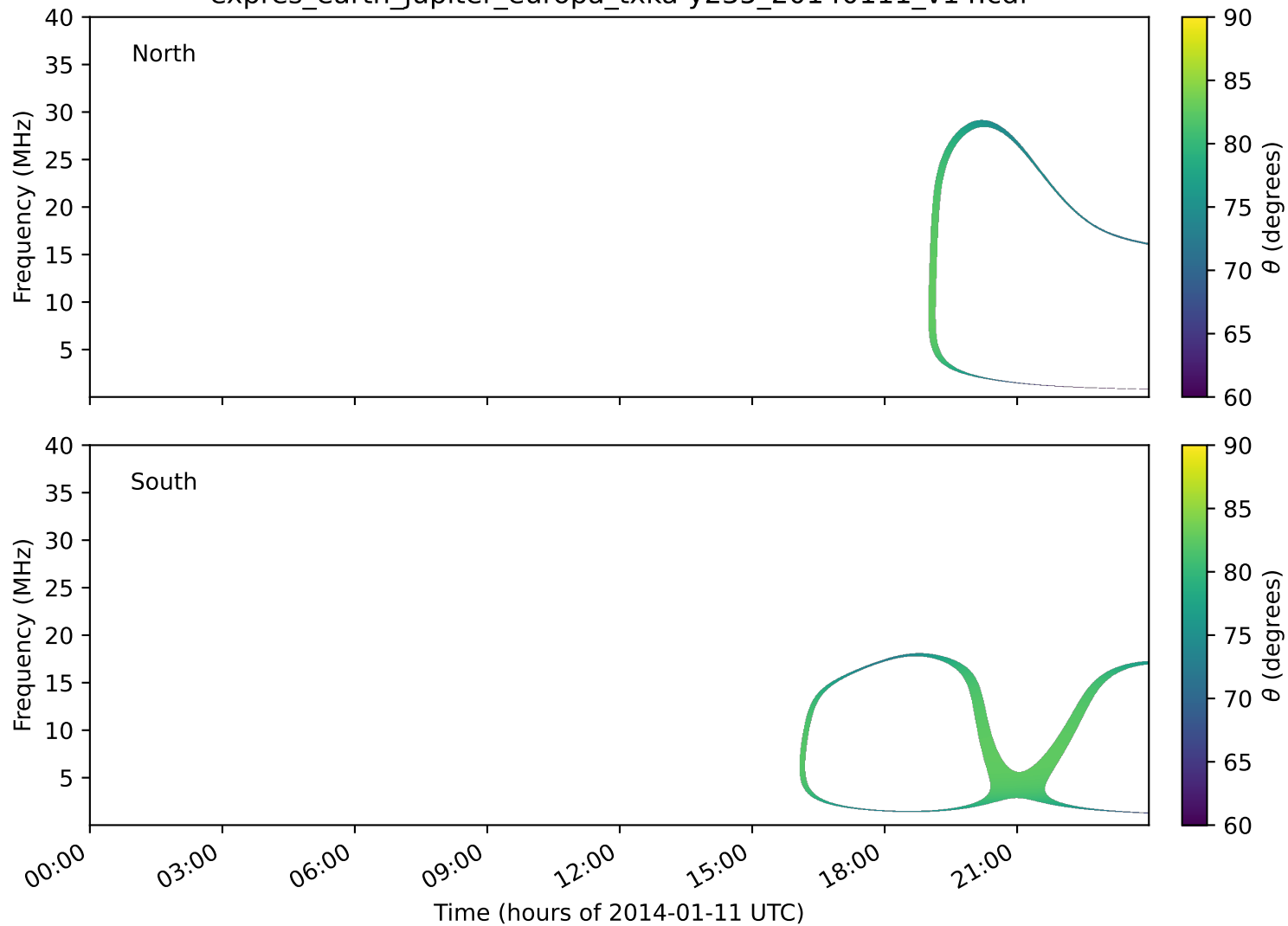
expres_earth_jupiter_europa_txka-y235_20140111_v14.cdf
