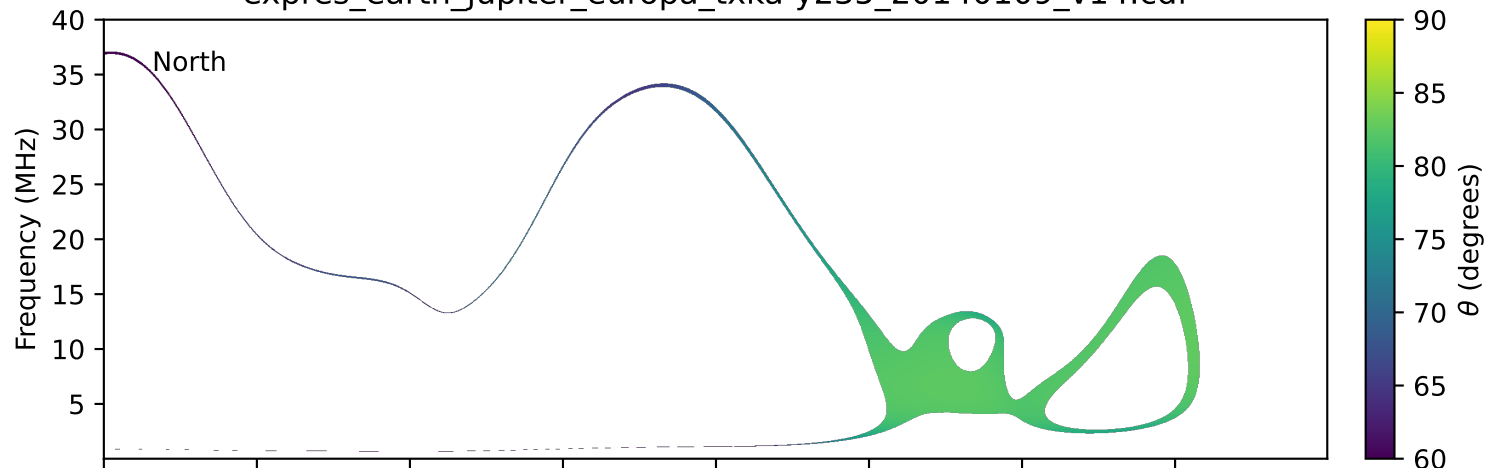
expres_earth_jupiter_europa_txka-y235_20140109_v14.cdf
