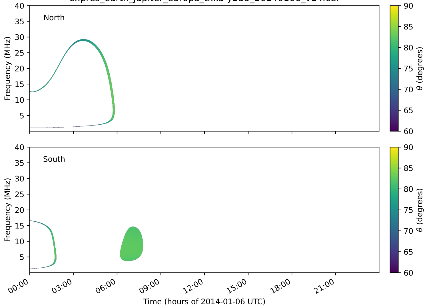
expres_earth_jupiter_europa_txka-y235_20140106_v14.cdf
