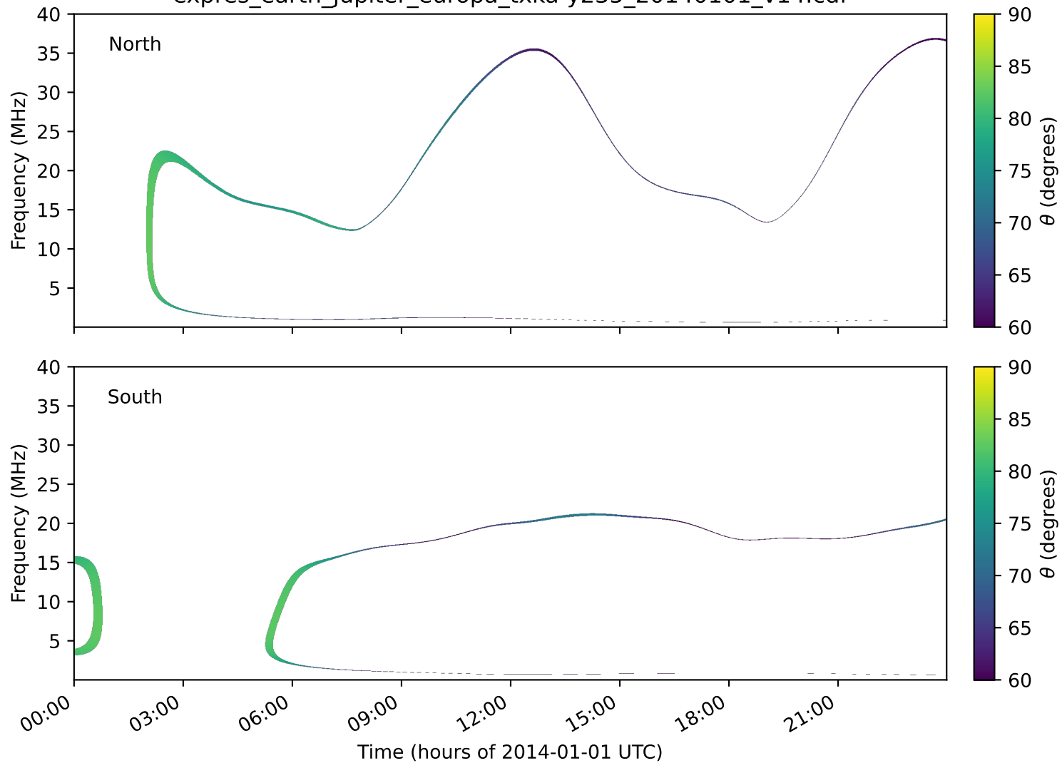
expres_earth_jupiter_europa_txka-y235_20140101_v14.cdf
