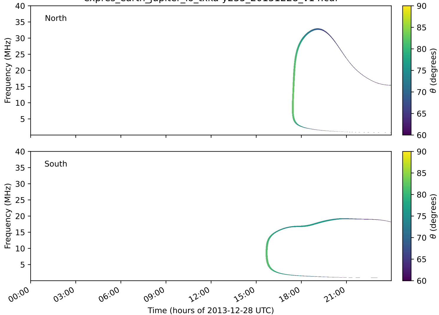
expres_earth_jupiter_io_txka-y235_20131228_v14.cdf
