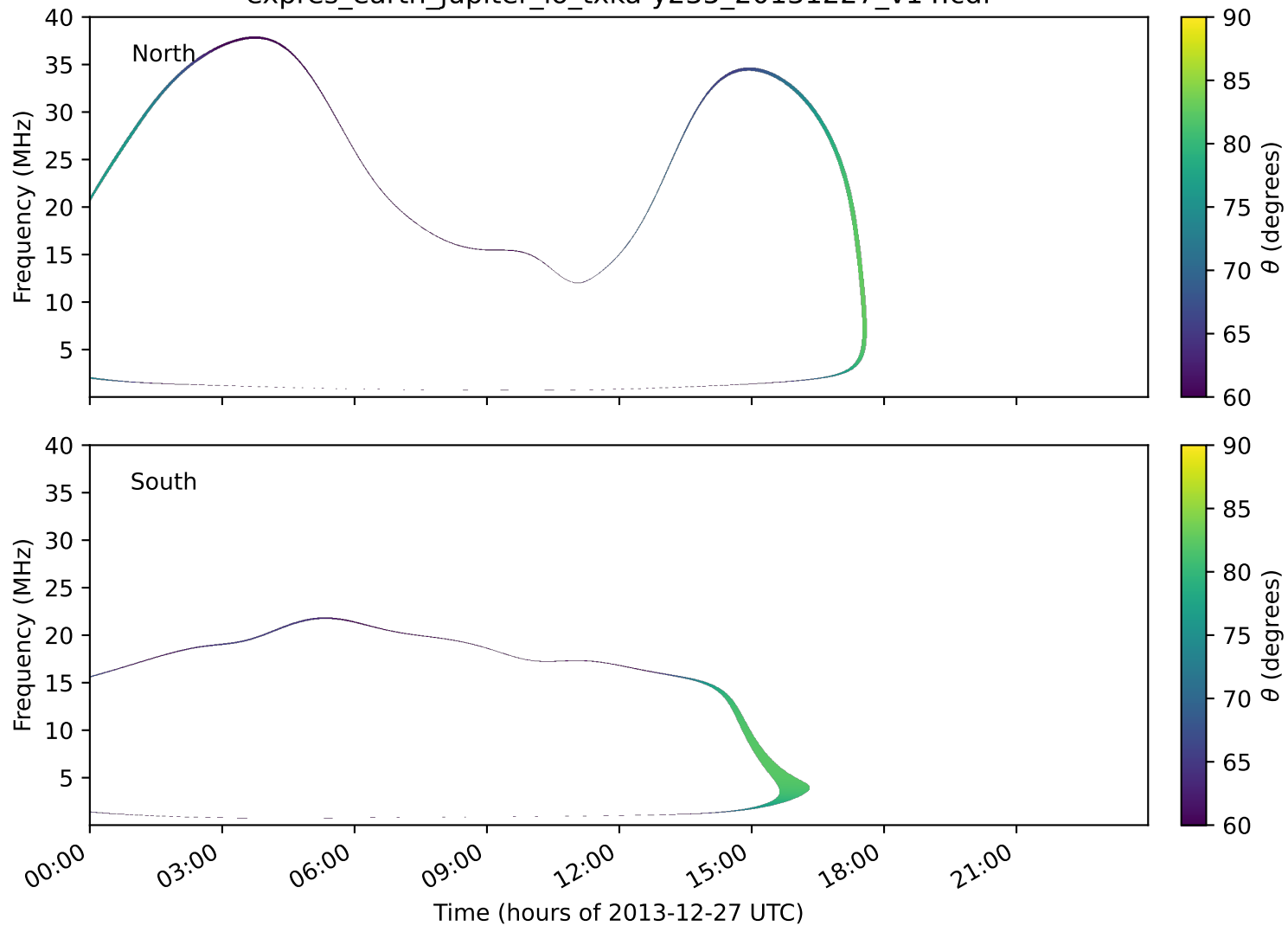
expres_earth_jupiter_io_txka-y235_20131227_v14.cdf
