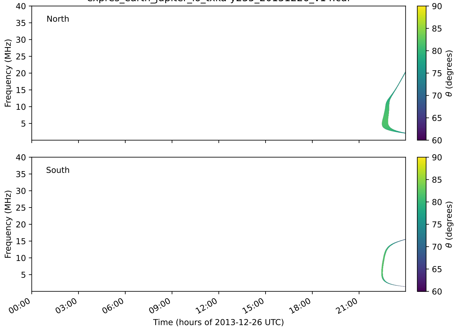
expres_earth_jupiter_io_txka-y235_20131226_v14.cdf
