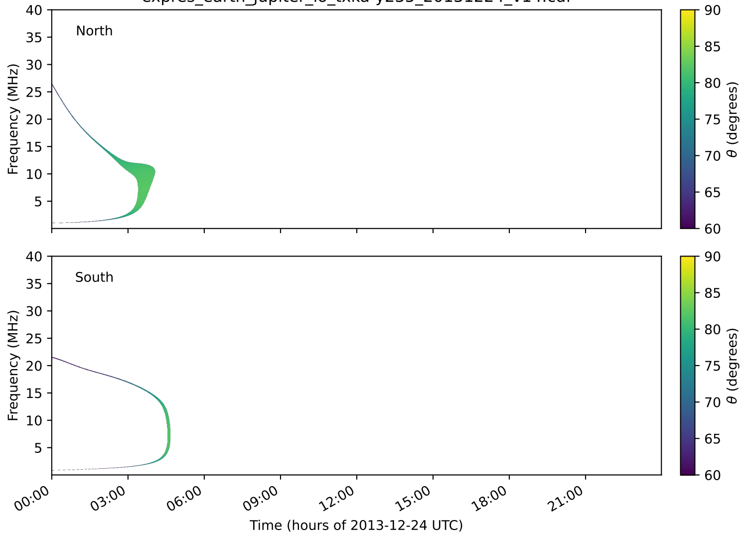
expres_earth_jupiter_io_txka-y235_20131224_v14.cdf
